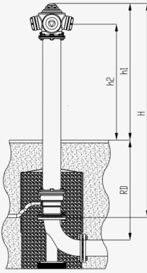
TYPE A – UNBREAKABLE CONSTRUCTION
