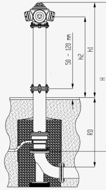
TYPE C – BREAKABLE CONSTRUCTION
